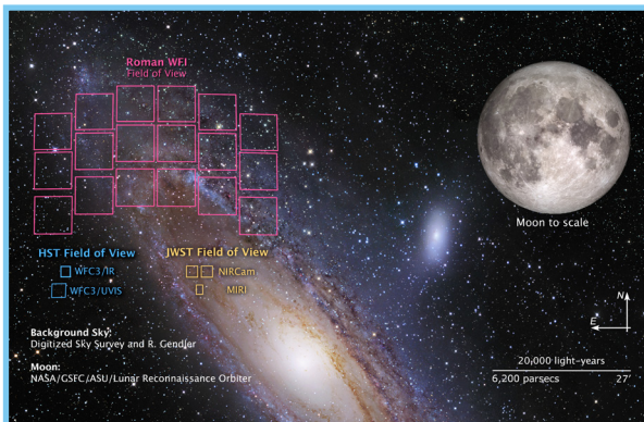
Roman's WFI consists of 18 near-IR detectors covering a total field of view of 0.281 square degrees.
