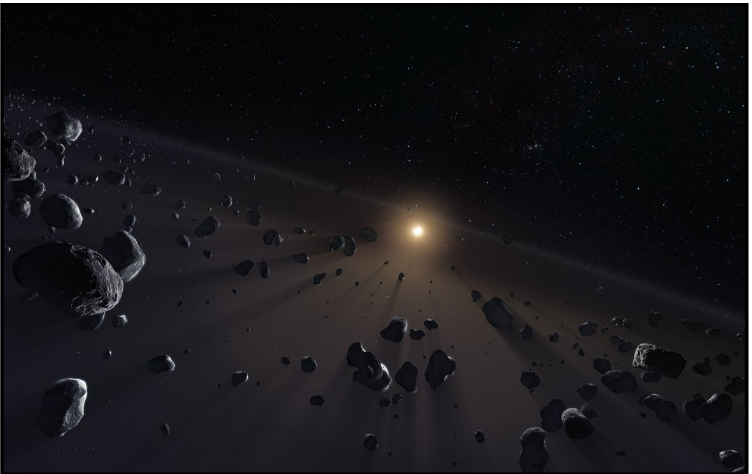
Illustration of objects in the Kuiper Belt. Credit: ESO/M. Kornmesser
