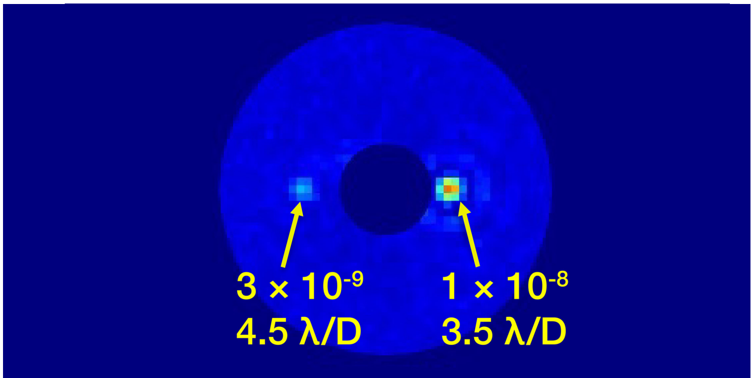
Simulated Roman Hybrid Lyot Coronagraph image of reflected visible light ( 0.575 \mu\text{m} ) from two exoplanets orbiting a G1V star ( V = 5 mag); labels indicate planet-to-star flux ratio and angular separation. Credit: Krist 2018, Observing Scenario 6
