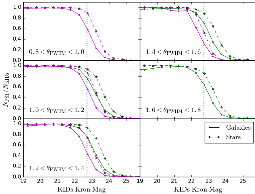
Both of the figures suggest the depth of the galaxy catalogue is typically 0.3-0.4 mags shallower than the stars.
