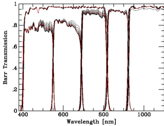
Figure 2. Filter transmission of the six Pan-STARRS1 filters. g_{P1} , r_{P1} , i_{P1} , z_{P1} , y_{P1} , and w_{P1} are shown as a function of field angle, in 0^\circ:15 steps to 1^\circ:65 , and the red curve shows the area-weighted average. Small field angles tend to have similar transmissions, allowing their curves to be distinguished from a large field angle.
